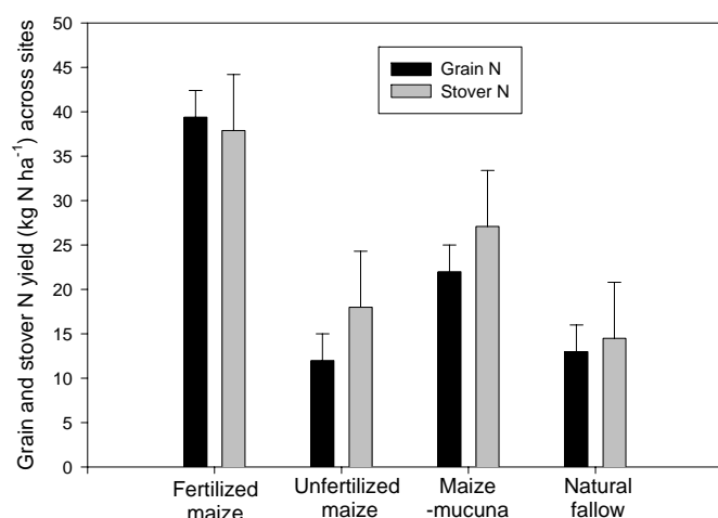
Figure 2. Maize grain and stover nitrogen from a maize-mucuna rotation, continuous maize and a natural fallow on 26 smallholder farms in central Malawi (From Sakala et al. 2003).
