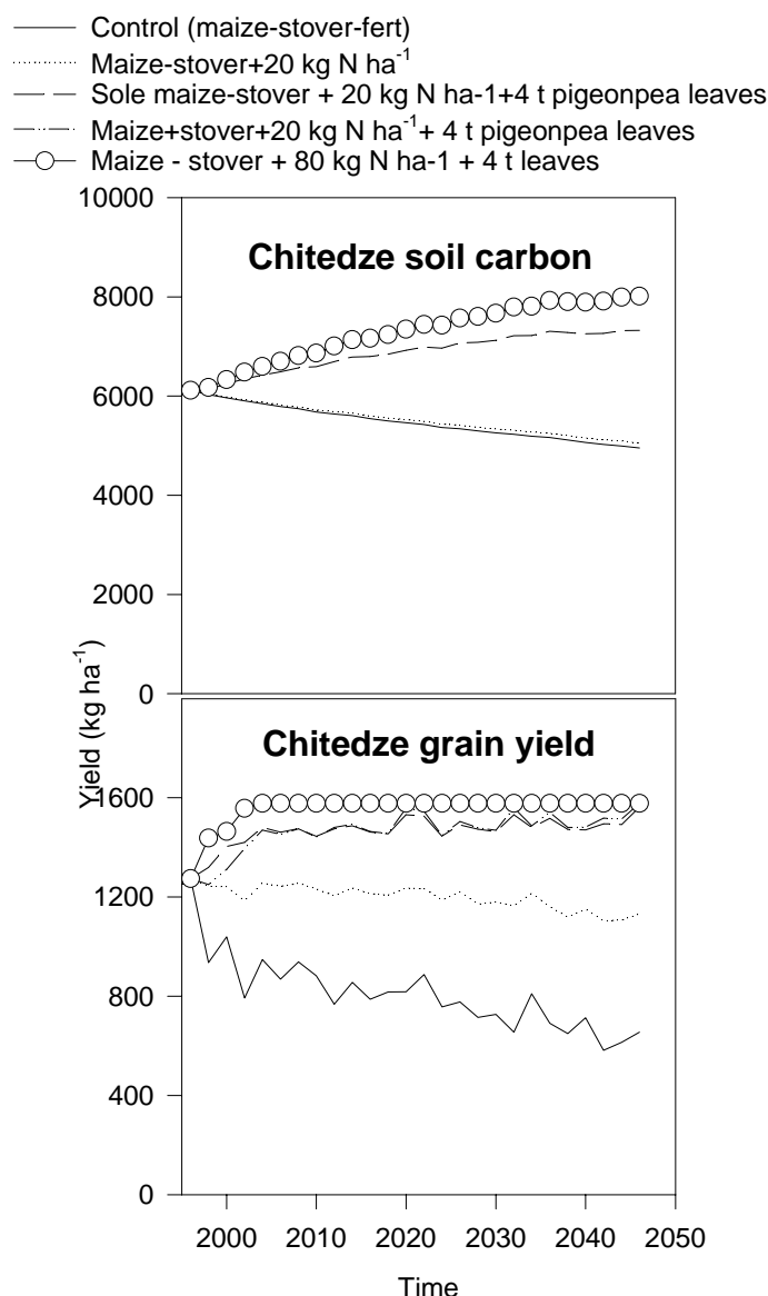
Figure 5. Fifty-year simulations of soil C and grain yield for maize-pigeonpea systems at Chitedze, Malawi using the CENTURY model.
