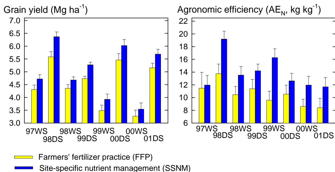
Figure 1. Gains in irrigated rice yield and the agronomic efficiency of fertilizer-N (kg grain yield increase per kg fertilizer-N applied) through site-specific nutrient management in Nueva Ecija province, Philippines. Values shown are means and standard errors of the same 27 fields managed from 1997 to 2001, including wet (WS) and dry (DS) season rice (Source: RTOP Project database, IRRI).
